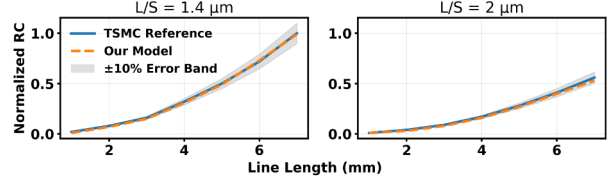
Fig. 14: RC scaling validation for organic RDL interposers.
